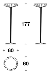
LBU (09) PIANTANA / STANDING LAMP Ø 60x177H.cm Ø 23 2/3x69 2/3H."
