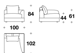
SHM (EDP) - SHM (ESP) ELEMENTO 1 POSTO CON BRACCIOLO DX O SX / 1 SEATER ELEMENT WITH RIGHT OR LEFT ARMREST 100x102x84H. - H.S.44cm 39 1/3x40x33H. - H.S.17 1/4"
