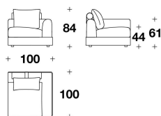
SHM (ANG) ELEMENTO ANGOLARE / CORNER ELEMENT 100x100x84H. - H.S.44cm 39 1/3x39 1/3x33H. - H.S.17 1/4"
