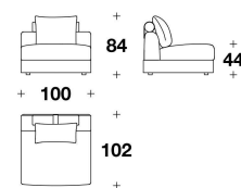
SHM (ECP) ELEMENTO CENTRALE / CENTRAL ELEMENT 100x102x84H. - H.S.44cm 39 1/3x40x33H. - H.S.17 1/4"
