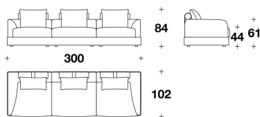
SHM (D4) DIVANO 4 POSTI / 4 SEATER SOFA 300x102x84H. - H.S.44cm 118x40x33H. - H.S.17 1/4"
