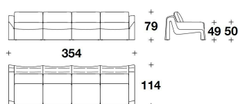
ING (D4) DIVANO 4 POSTI / 4 SEATER SOFA 354x114x79H. - H.A.50 - H.S.49cm 139 1/2x45x31H. - H.A.19 3/4 - H.S.19 1/4"
