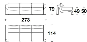
ING (D3) DIVANO 3 POSTI / 3 SEATER SOFA 273x114x79H. - H.A.50 - H.S.49cm 107 1/3x45x31H. - H.A.19 3/4 - H.S.19 1/4"
