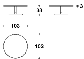
CTD (25M) - CTD (25) - CTD (25R) COFFEE TABLE Ø 103x38H.cm Ø 40 2/3x15H. "
