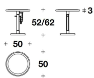
CTD (18M) - CTD (18) - CTD (18R) SIDE TABLE Ø 50x52-62H.cm Ø 19 3/4x20 1/3-24 1/3H. "
