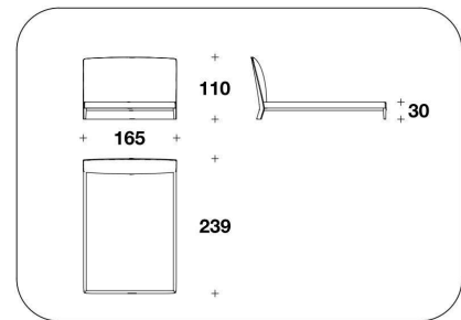
NWE (EQUSA) VENEERED - QUEEN USA : LETTO PER MATERASSO / BED FOR MATTRESS 152x205 - 165x239x110H. - H.B.30cm 60x80 2/3 - 65x94x43 1/3H. - H.B.11 3/4"
