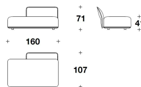
NAT (ECD) - NAT (ECS) ELEMENTO CON SCHIENALE DX O SX / SEAT ELEMENT WITH RIGHT OR LEFT BACK 160x107x71H. - H.S.41cm 63x42x28H. - H.S.16 1/4"
