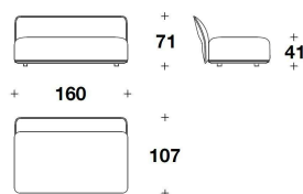
NAT (EC) ELEMENTO CENTRALE / CENTRAL ELEMENT 160x107x71H. - H.S.41cm 63x42x28H. - H.S.16 1/4"
