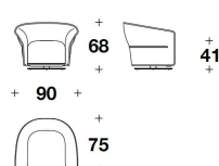
NAT (POL) POLTRONA / ARMCHAIR 90x75x68H. - H.S.41cm 35 1/3x29 2/3x26 2/3H. - H.S.16 1/4"
