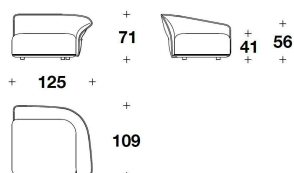
NAT (EDG) - NAT (ESG) BIG : ELEMENTO CON BRACCIOLO DX O SX / ELEMENT WITH RIGHT OR LEFT ARMREST 125x109x71H. - H.S.41cm 49 1/3x43x28H. - H.S.16 1/4"
