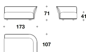
NAT (ANGD) - NAT (ANGS) ELEMENTO ANGOLARE DX O SX / RIGHT OR LEFT CORNER ELEMENT 173x107x71H. - H.S.41cm 68x42x28H. - H.S.16 1/4"
