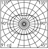
Luminous flux luminaire 1530 lm
