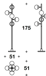
TRL (09) PIANTANA / STANDING LAMP 51x51x175H.cm 20x20x69H."
